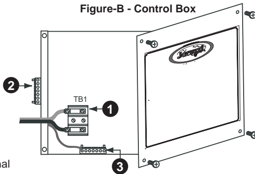
Figure-B - Control Box
